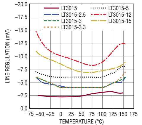
Line Regulation
