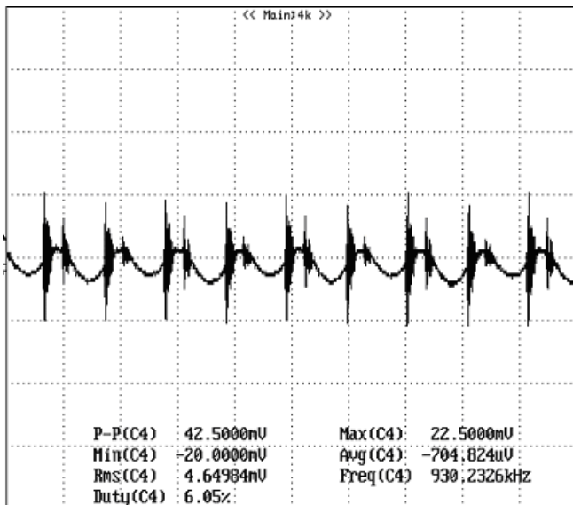
Figure 15: Output voltage ripple at nominal input voltage and rated load current ( I_o=10\text{A} ) (20 mV/div, 2 μs/div) Load capacitance: 1\mu\text{F} ceramic capacitor and 10\mu\text{F} tantalum capacitor. Bandwidth: 20 MHz. Scope measurements should be made using a BNC cable (length shorter than 20 inches). Position the load between 51 mm to 76 mm (2 inches to 3 inches) from the module.
