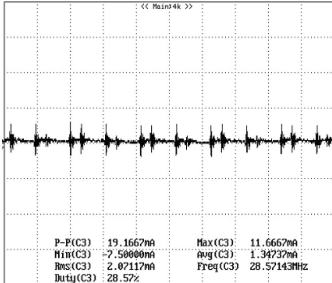
Figure 13: Input reflected ripple current, i_s , through a 12\mu\text{H} source inductor at nominal input voltage and rated load current (20 mA/div, 2 μs/div).
