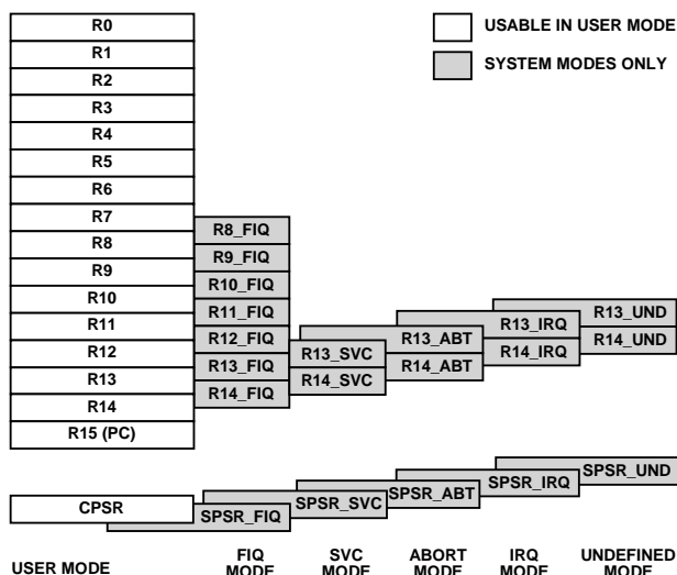
Figure 15. Register Organization
