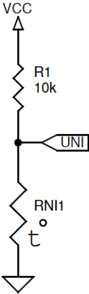
Example of voltage dividing circuit using Ni1000SOT sensor
