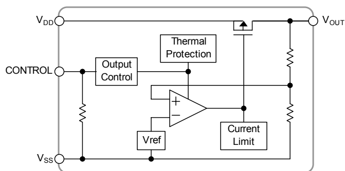
NJU7771/72/73
