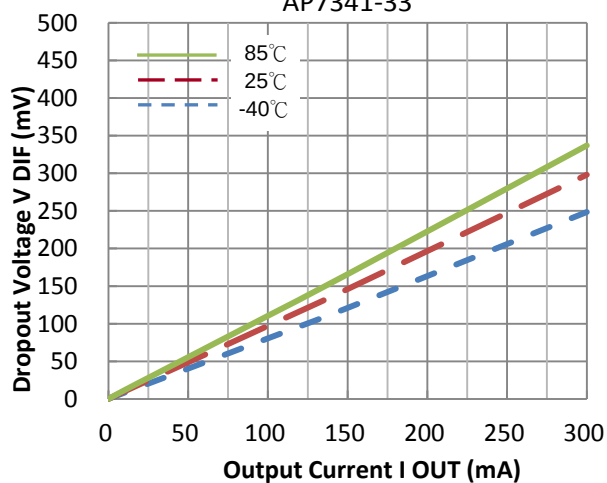
Dropout Voltage vs. Output Current AP7341-33
