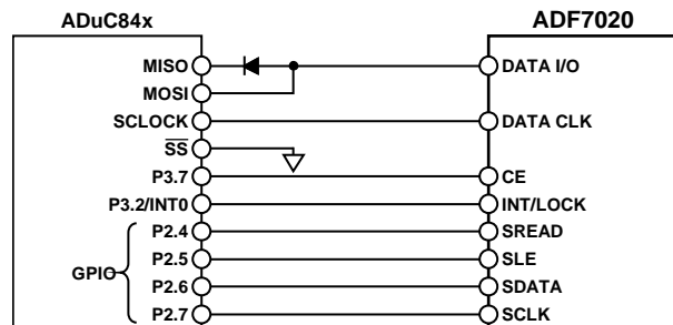
Figure 37. ADuC84x to ADF7020 Connection Diagram
