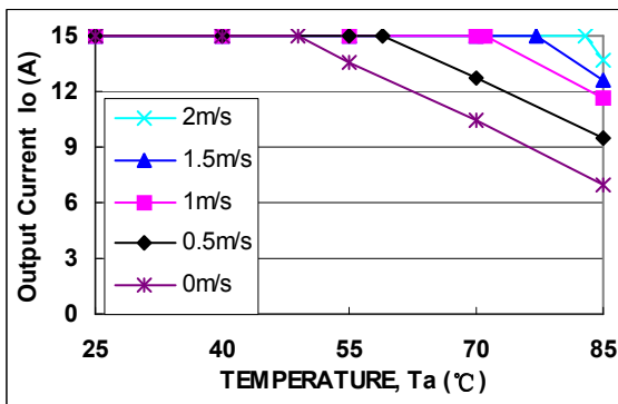
Fig. 88 AVO75-48S05 output power derating Airflow direction from -Vin to +Vin; Vin=48V
