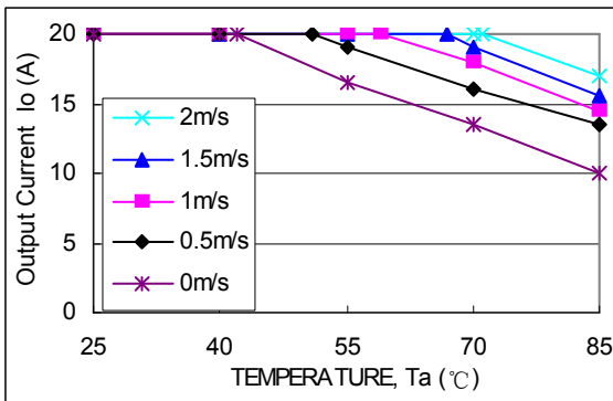
Fig. 87 AVO75-48S3V3 output power derating Airflow direction from -Vin to +Vin; Vin=48V
