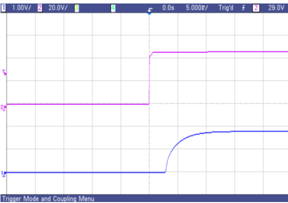
Fig. 61 AVO75-48S1V8 typical start-up from power on
