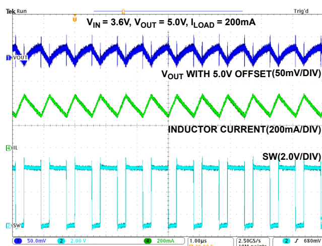
FIGURE 18. PWM WAVEFORM
