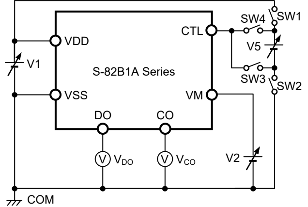
Figure 5 Test Circuit 2
