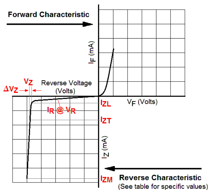
FIGURE 4 Zener Diode Characteristics and Symbol Identification
