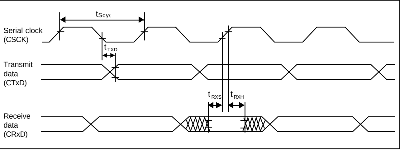
Figure 17-17. SCI Input/Output Timing (Synchronous Mode)
