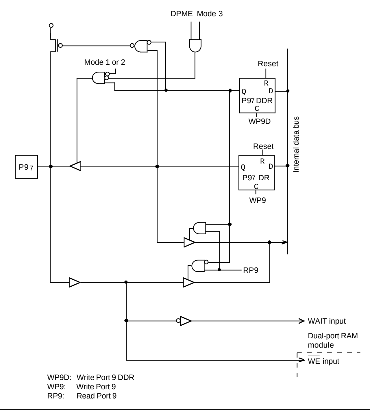
Figure 5-25. Port 9 Schematic Diagram (Pin P97)
