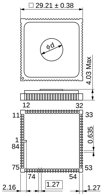
Figure E-1. Package Dimensions (CG-84)
