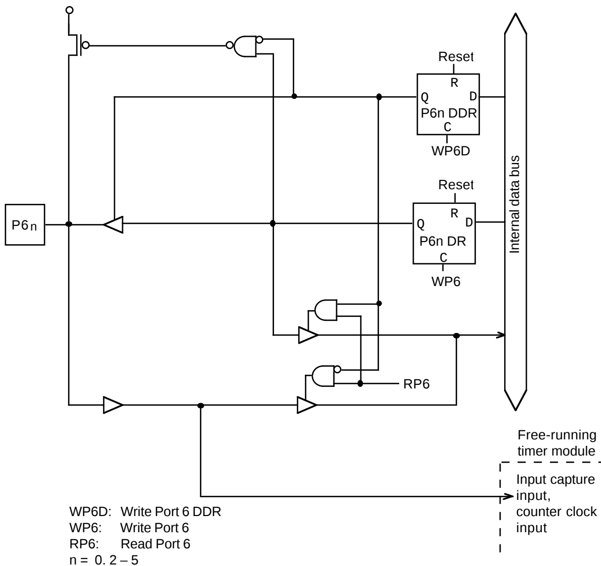
Figure 5-9. Port 6 Schematic Diagram (Pins P60, P62, P63, P64, and P65)
