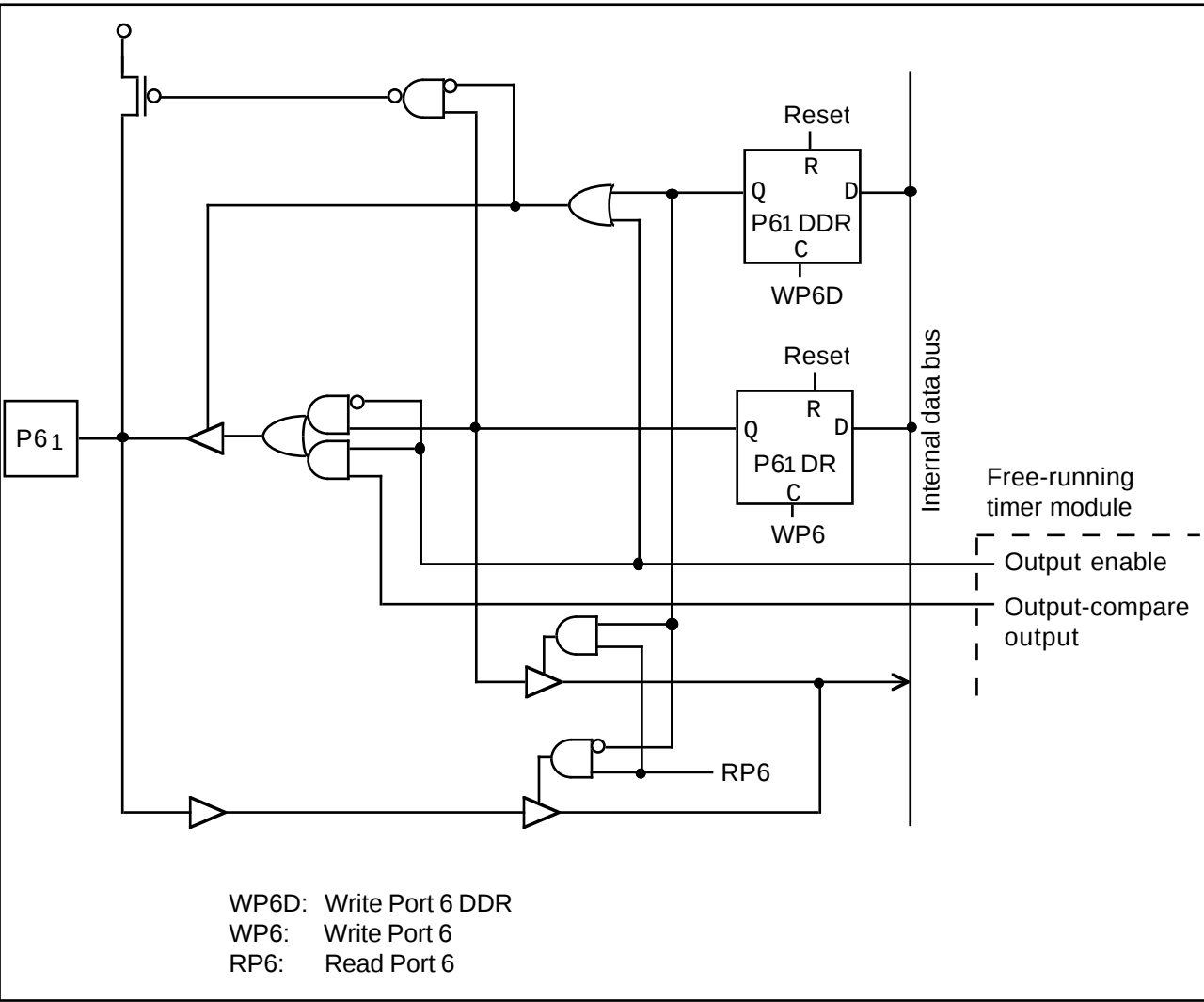
Figure 5-10. Port 6 Schematic Diagram (Pin P61)
