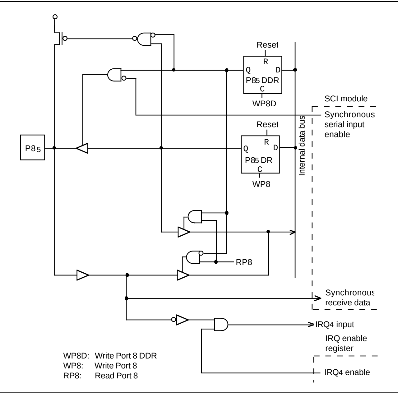
Figure 5-18. Port 8 Schematic Diagram (Pin P85)
