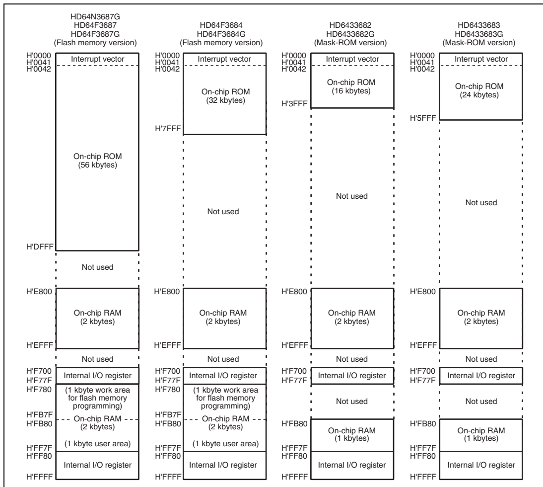
Figure 2.1 Memory Map (1)
