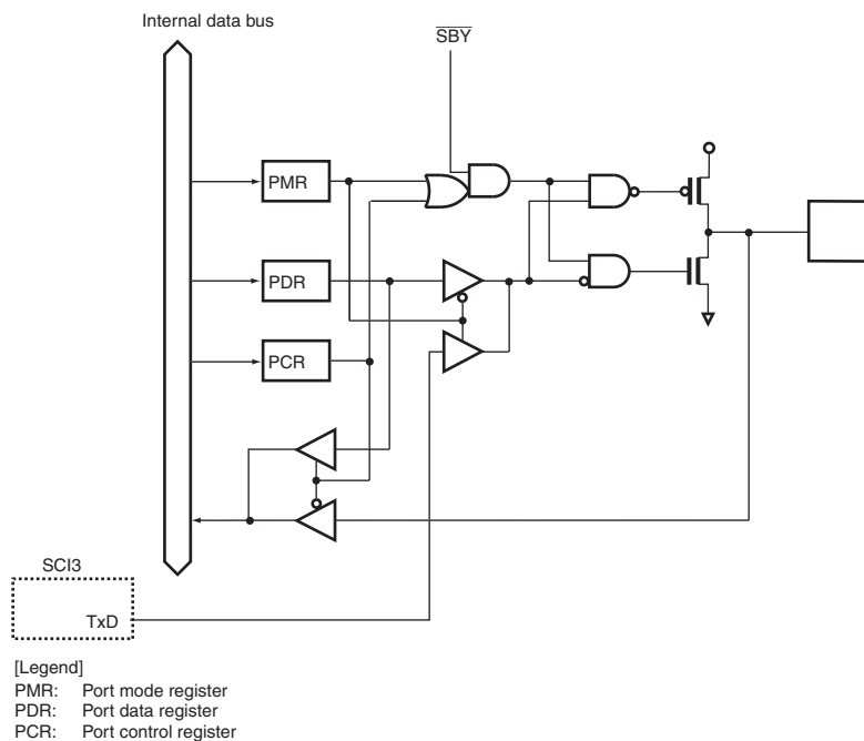
Figure B.8 Port 2 Block Diagram (P22)
