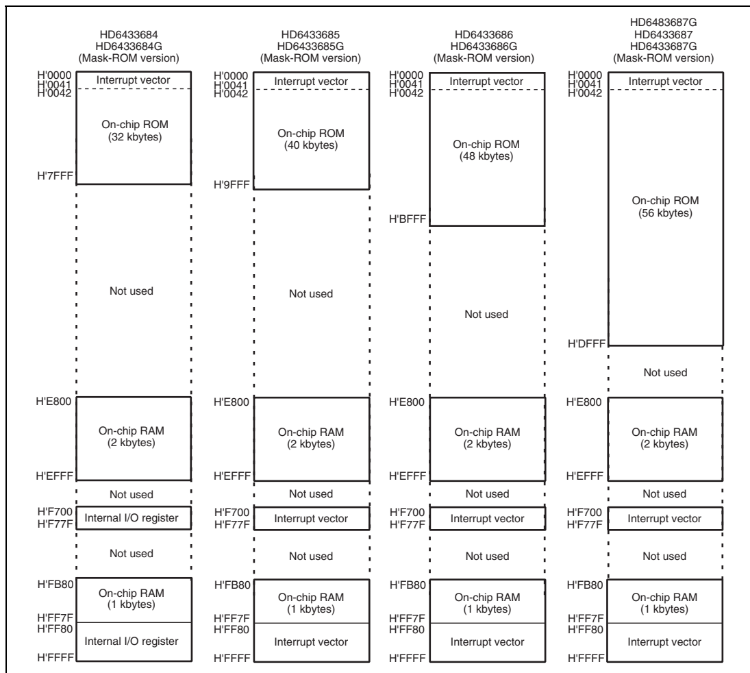
Figure 2.1 Memory Map (2)
