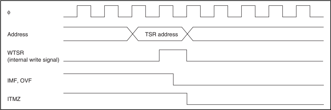
Figure 13.51 Status Flag Clearing Timing
