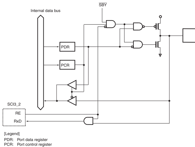
Figure B.20 Port 7 Block Diagram (P71)
