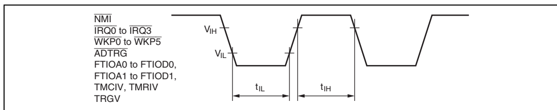
Figure 23.3 Input Timing
