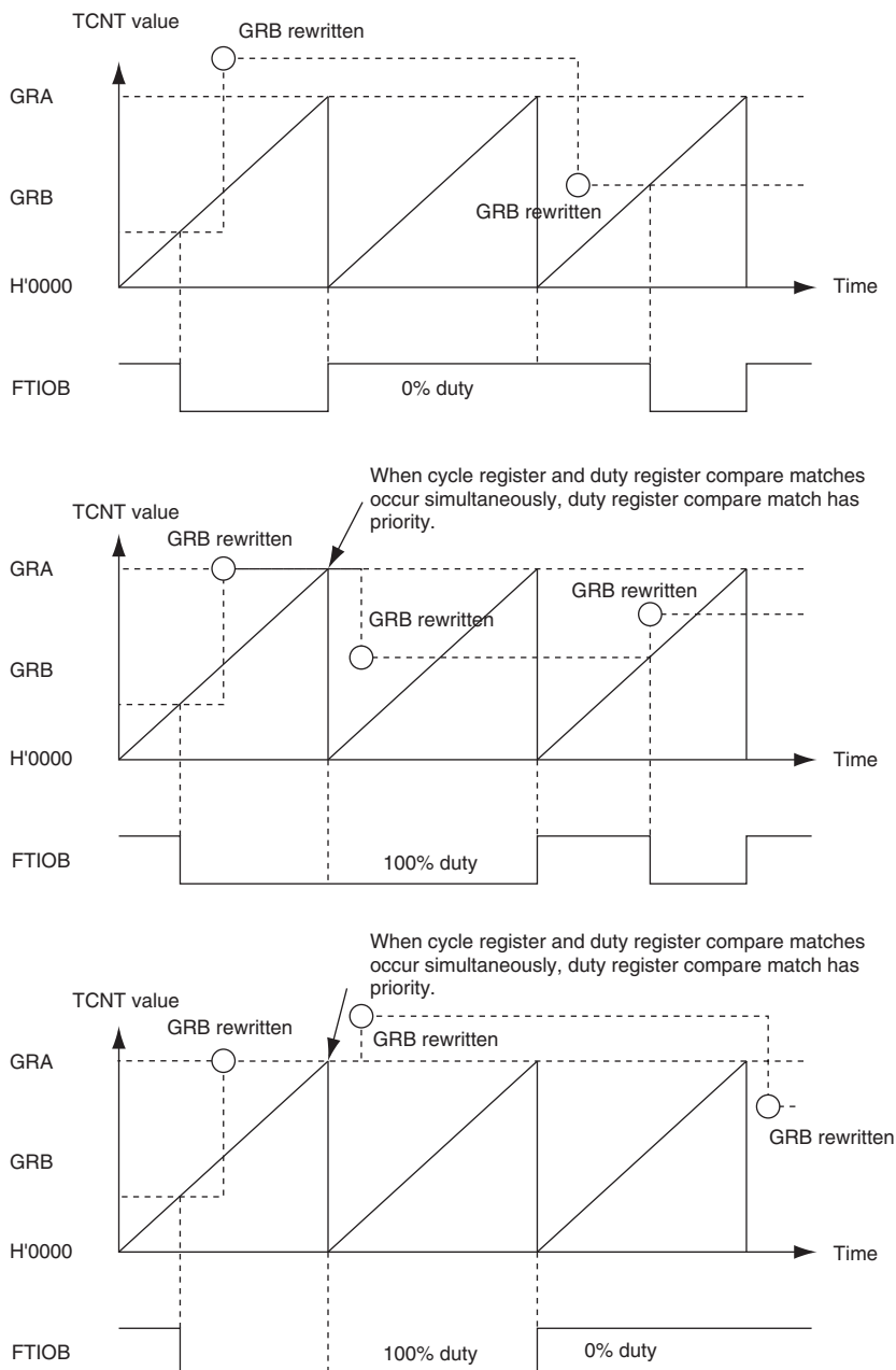
Figure 13.24 Example of PWM Mode Operation (3)
