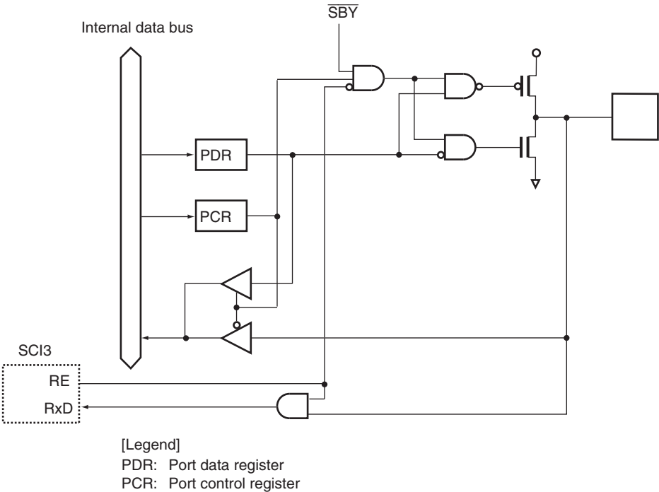
Figure B.9 Port 2 Block Diagram (P21)
