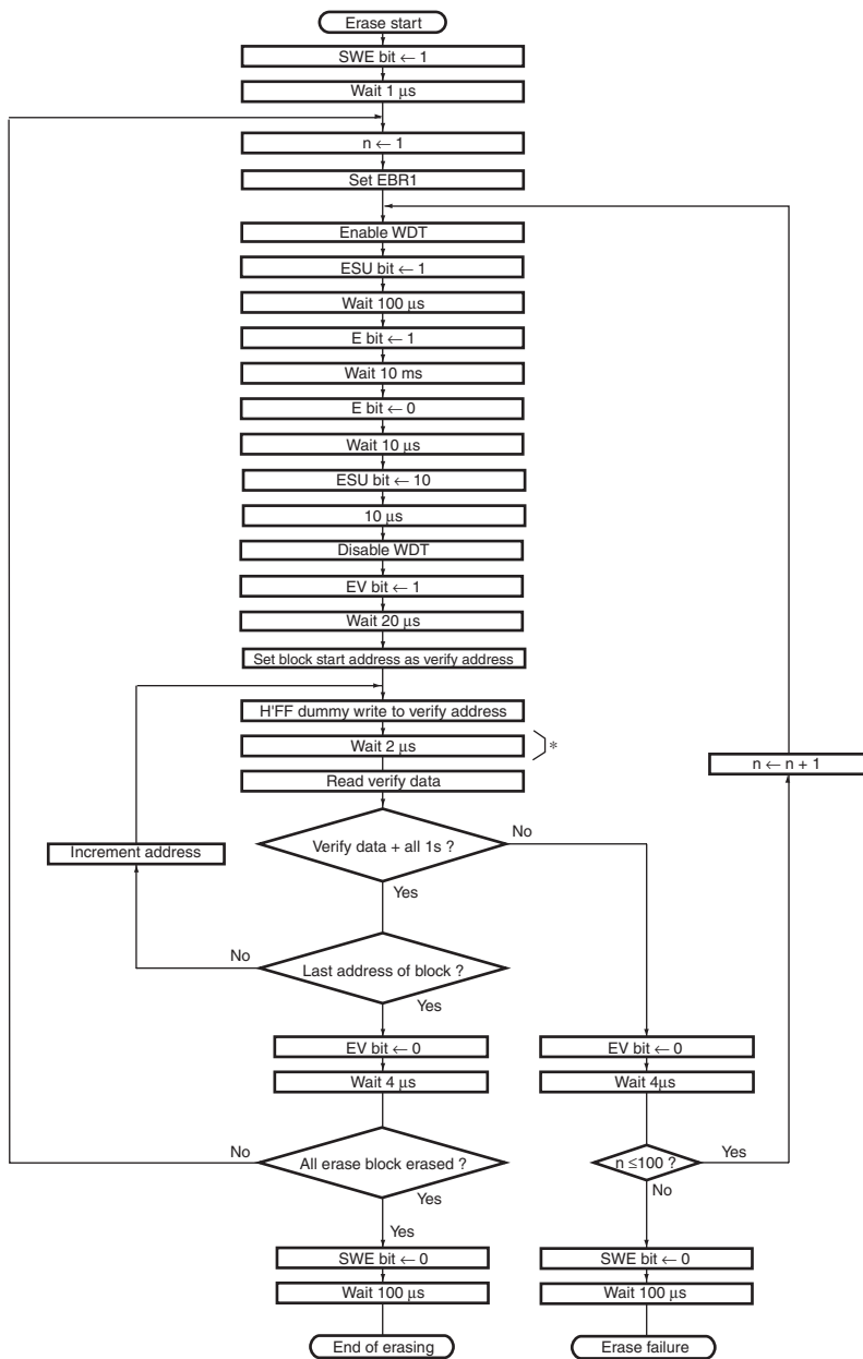
Figure 7.4 Erase/Erase-Verify Flowchart
