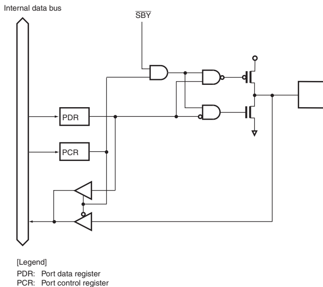
Figure B.11 Port 3 Block Diagram (P37 to P30)
