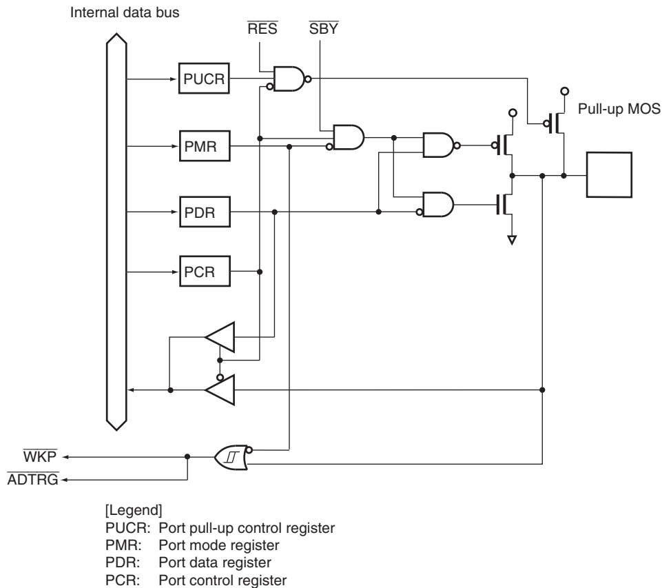
Figure B.13 Port 5 Block Diagram (P55)
