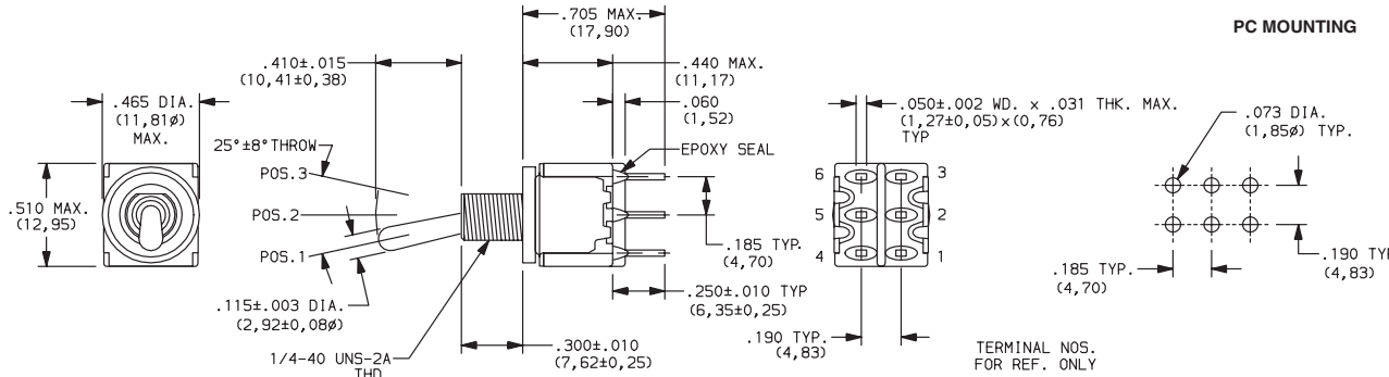
DPDT
