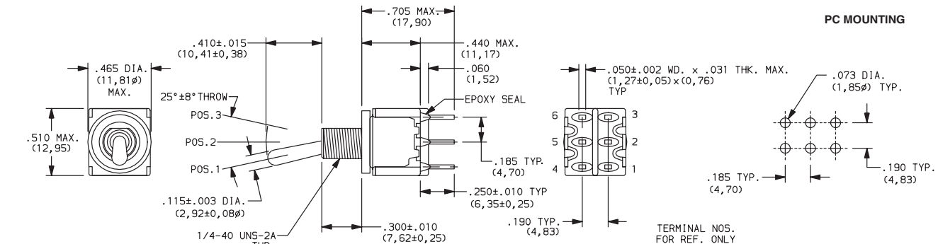
DPDT
