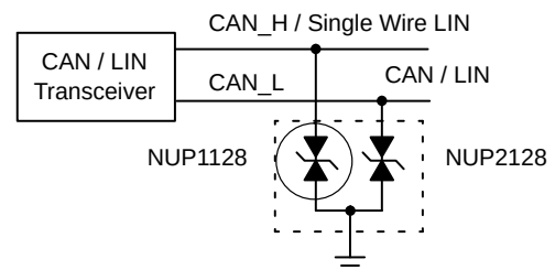
NUP2128
