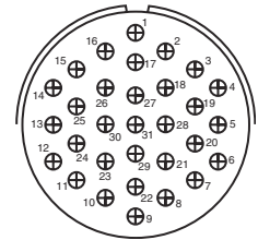
32-31 Service Rating A Number of Contacts 31 Contact Size 16
