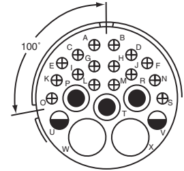
32-16 Service Rating A Number of Contacts 2 3 2 16 Contact Size 4 8 12 16
