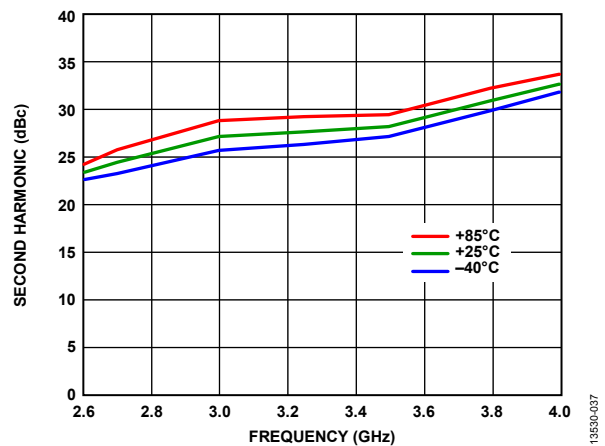
Figure 37. Second Harmonic vs. Frequency at Various Temperatures, P_{OUT} = 30 \text{ dBm}
