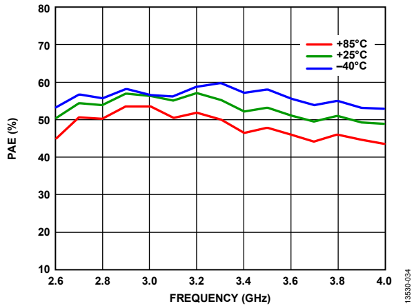
Figure 34. Power Added Efficiency (PAE) vs. Frequency at Various Temperatures, P_{IN} = 16 \text{ dBm}
