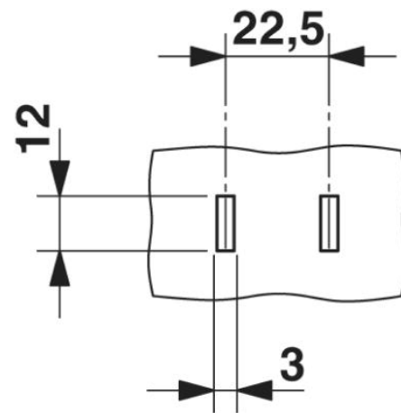
Punching template
