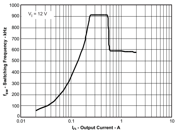
Figure 18. \text{VO1}=3.3\text{V} , SW-frequency vs Output Current
