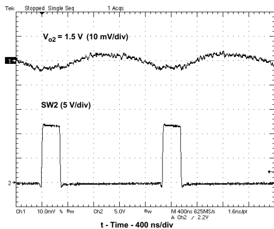
Figure 21. \text{VO2}=1.5\text{ V} , Ripple Voltage ( I_{O2}=2\text{ A} )
