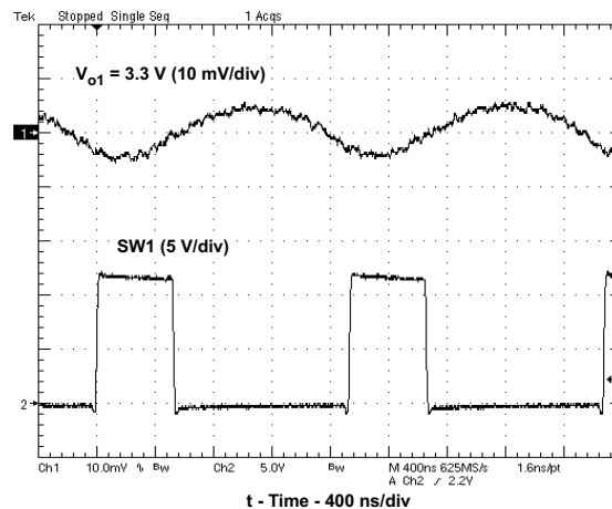
Figure 20. \text{VO1}=3.3\text{ V} , \text{VO1} Ripple Voltage ( I_{O1}=2\text{ A} )
