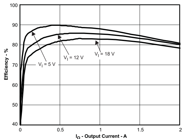
Figure 14. \text{VO1}=1.5\text{V} , Efficiency vs Output Current
