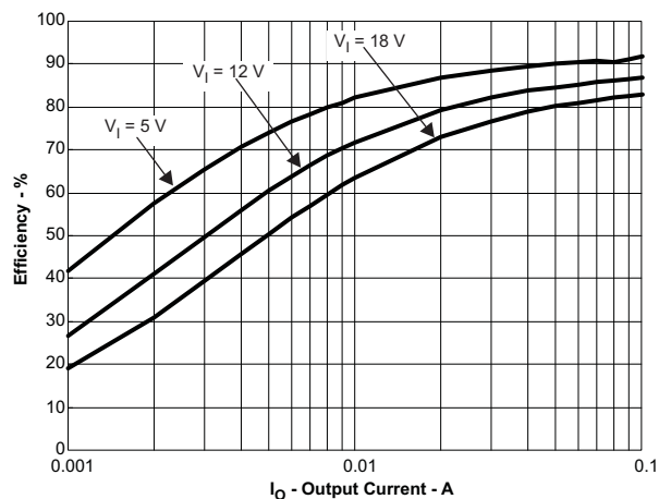
Figure 13. \text{VO1}=3.3\text{V} , Efficiency vs Output Current
