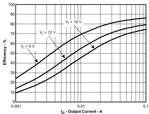
Figure 15. \text{VO2}=1.5\text{V} , Efficiency vs Output Current
