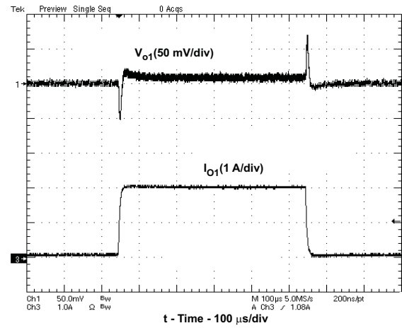
Figure 8. \text{VO1}=3.3\text{V} , 0A to 2A Load Transient Response
