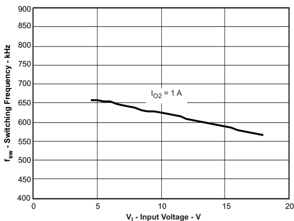
Figure 17. \text{VO2}=1.5\text{V} , SW-frequency vs Input Voltage
