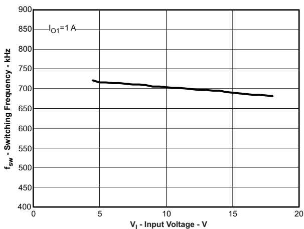
Figure 16. \text{VO1}=3.3\text{V} , SW-frequency vs Input Voltage
