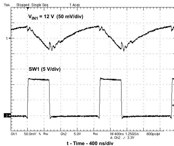
Figure 22. \text{VIN1} Input Voltage Ripple ( I_{O1}=2\text{ A} )
