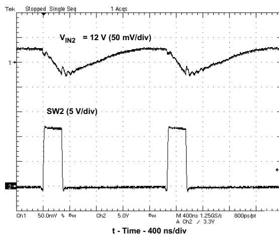
Figure 23. \text{VIN2} Input Voltage Ripple ( I_{O2}=2\text{ A} )
