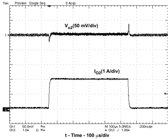
Figure 9. \text{VO2}=1.5\text{V} , 0A to 2A Load Transient Response
