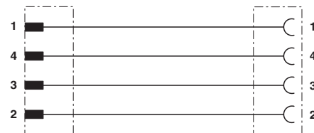
Contact assignment of the M8/M12 adapter
