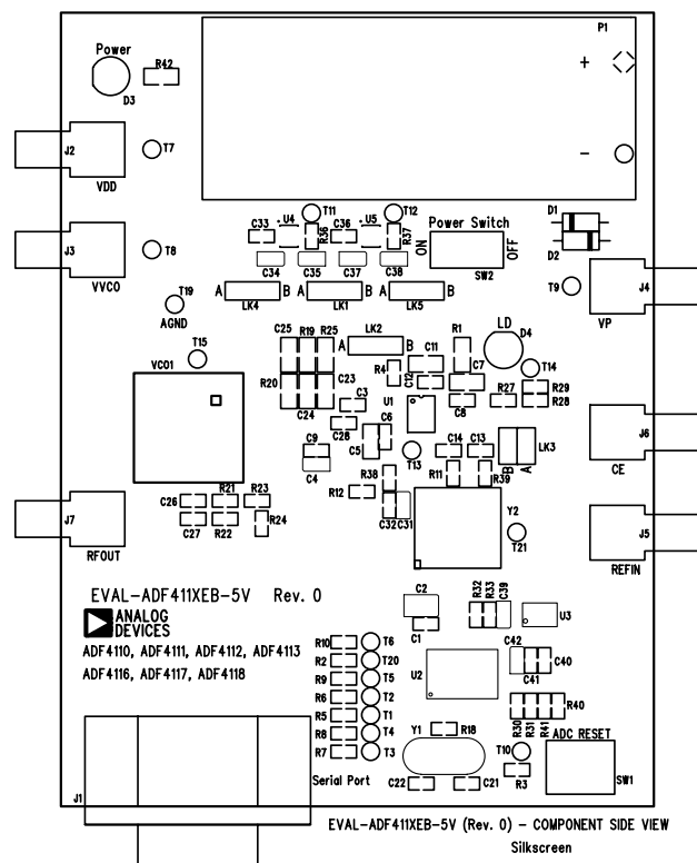
Figure 1. Evaluation Board Silkscreen
