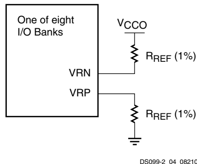
Figure 9: Connection of Reference Resistors ( R_{REF} )
