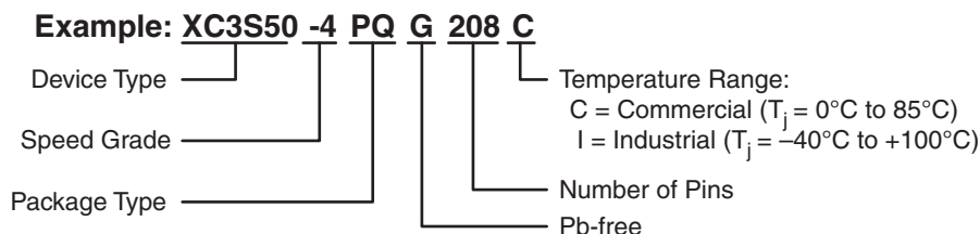
Figure 6: Pb-Free Packaging
