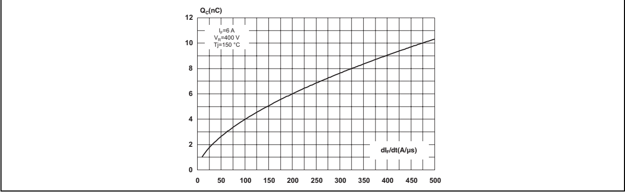
Figure 7. Total capacitive charges versus dl_F/dt (typical values)
