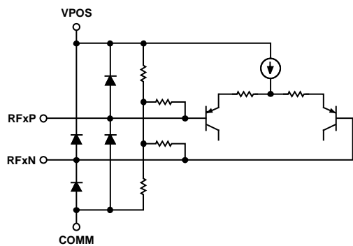
Figure 6. RF Inputs
