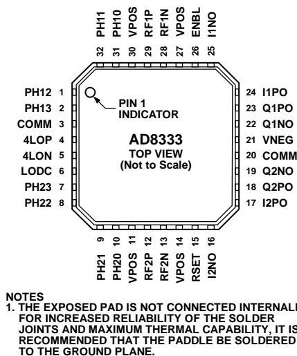
Figure 2. 32-Lead LFCSP Pin Configuration
