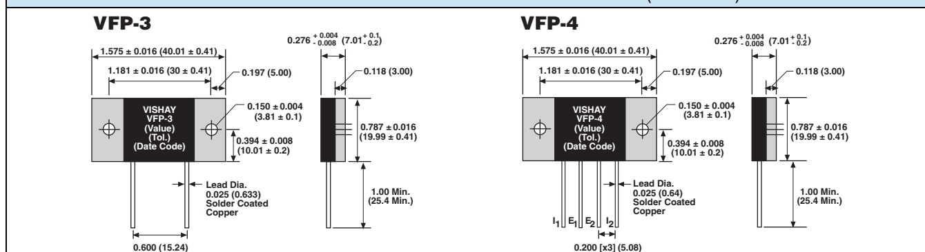
FIGURE 1 - STANDARD IMPRINTING AND DIMENSIONS in inches (millimeters)
