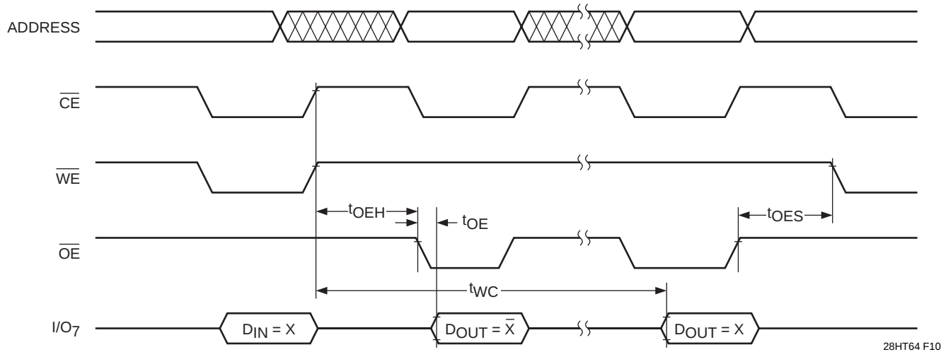
Figure 7. \overline{\text{DATA}} Polling
