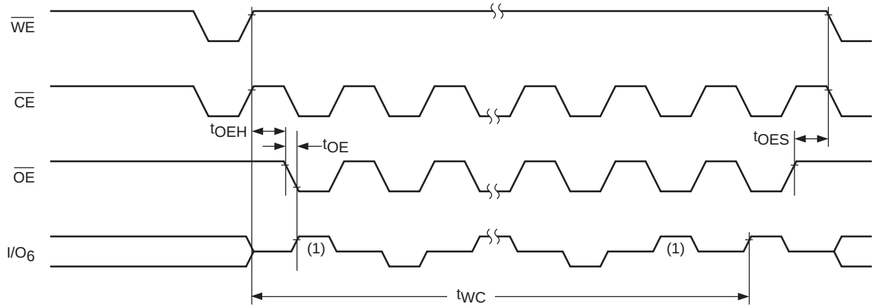
Figure 8. Toggle Bit
