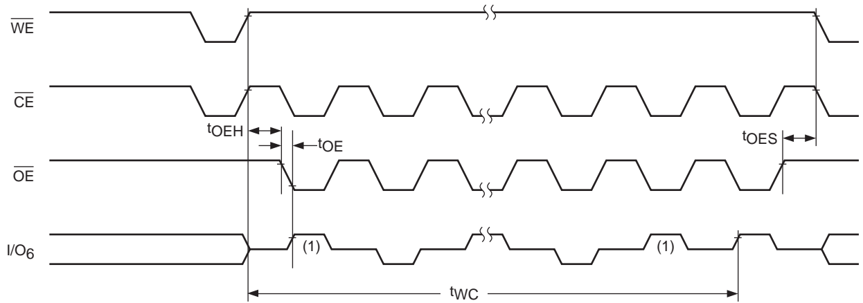
Figure 8. Toggle Bit
