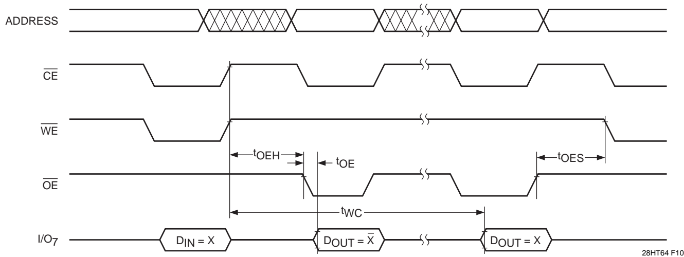
Figure 7. DATA Polling
