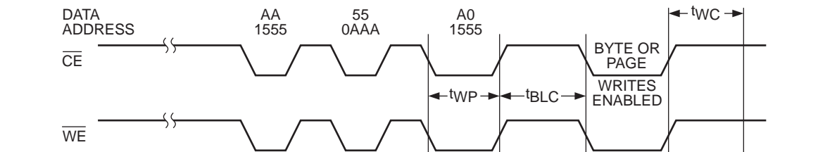
Figure 11. Software Data Protection Timing
