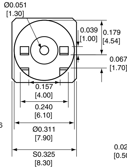
BACK VIEW
