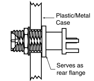
MOUNTING METHODS
