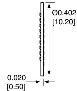
WASHER
