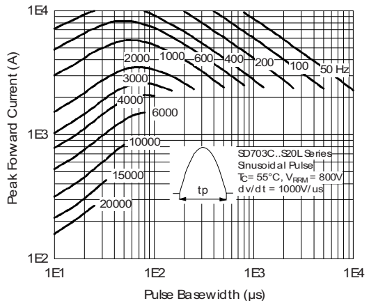
Fig. 29 - Frequency Characteristics
