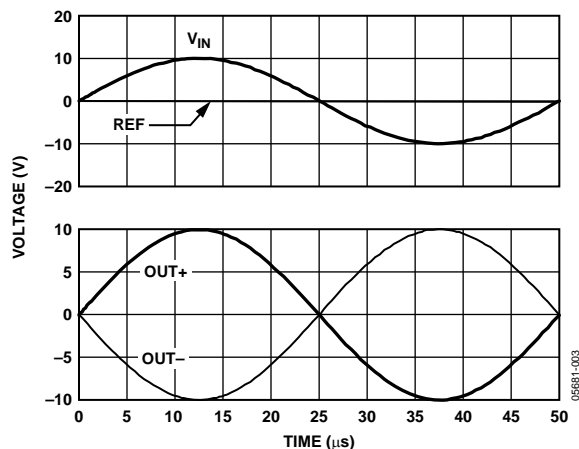
Figure 42. Typical Input/Output Response—Centered Reference
