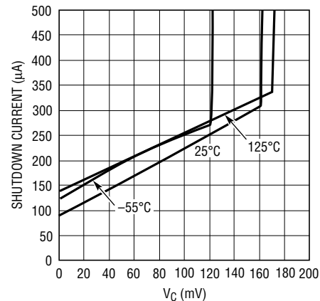
Shutdown Supply Current vs V_C Voltage
