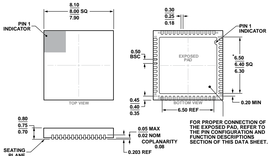
Figure 44. 56-Lead Lead Frame Chip Scale Package [LFCSP_WQ] 8 mm x 8 mm Body, Very Very Thin Quad (CP-56-10) Dimensions shown in millimeters
