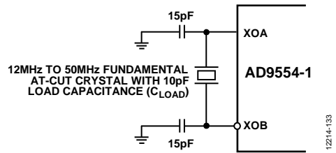
Figure 24. System Clock Input (XOA/XOB) in Crystal Mode (The recommended C_{LOAD} = 10\text{ pF} is shown. The 15\text{ pF} shunt capacitors shown in this figure must equal 2 \times (C_{LOAD} - C_{STRAY}) , where C_{STRAY} is typically 2\text{ pF} to 5\text{ pF} .)
