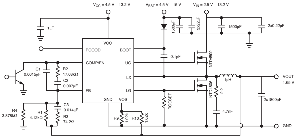
NCP1589A Application Diagram
