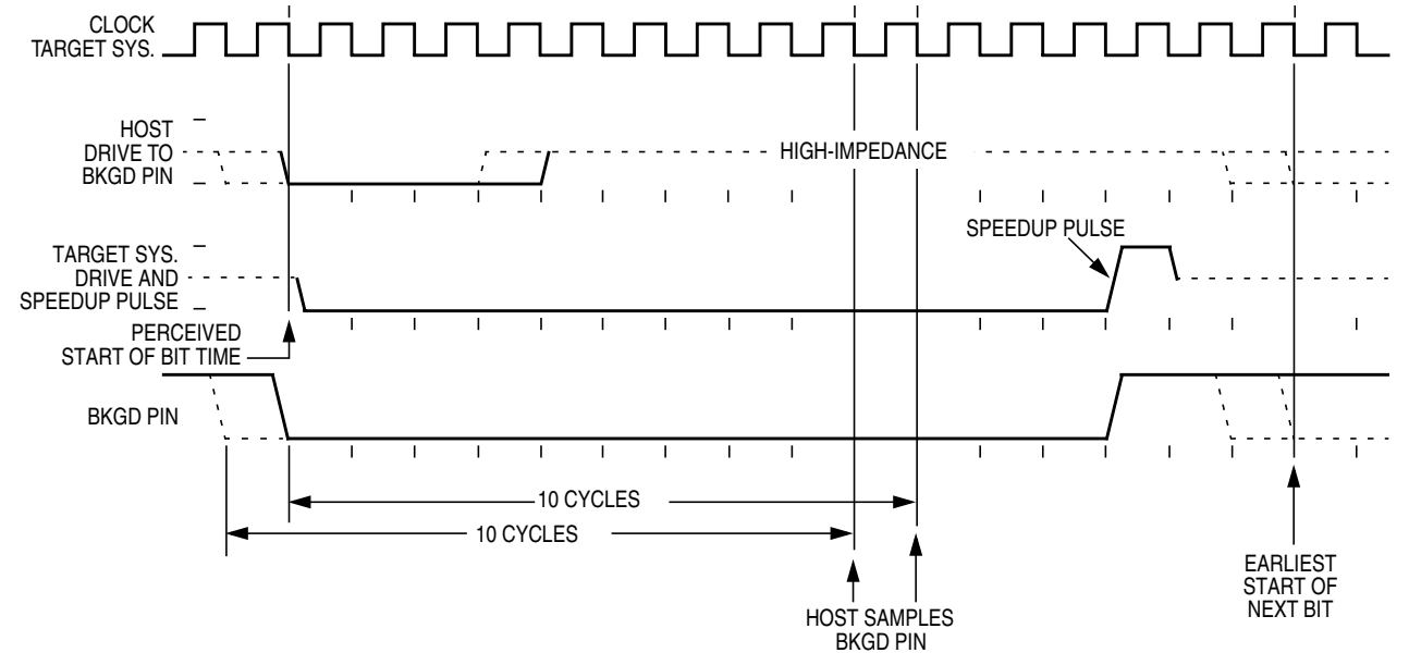
Figure 6-9. BDM Target-to-Host Serial Bit Timing (Logic 0)
