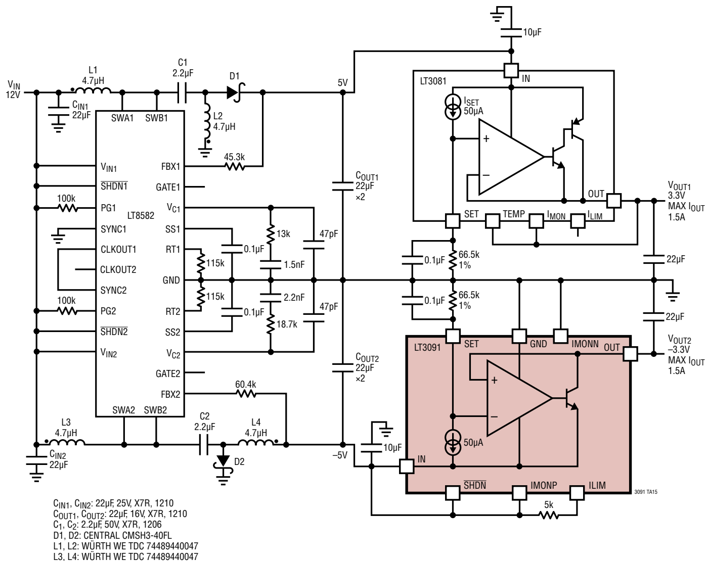
12V to \pm 3.3\text{V} Low Noise Power Supply
