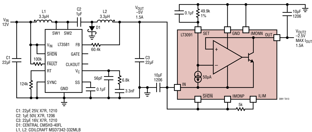
Low Noise Single Inductor Positive-to-Negative Converter
