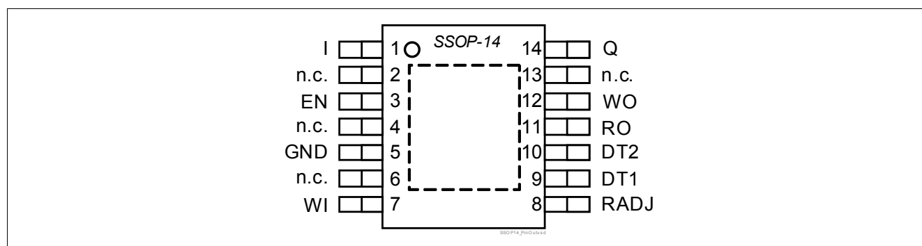
Figure 3 Pin Configuration
