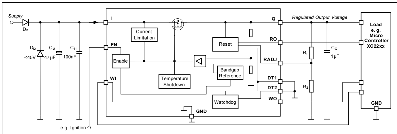
Figure 13 Application Diagram
