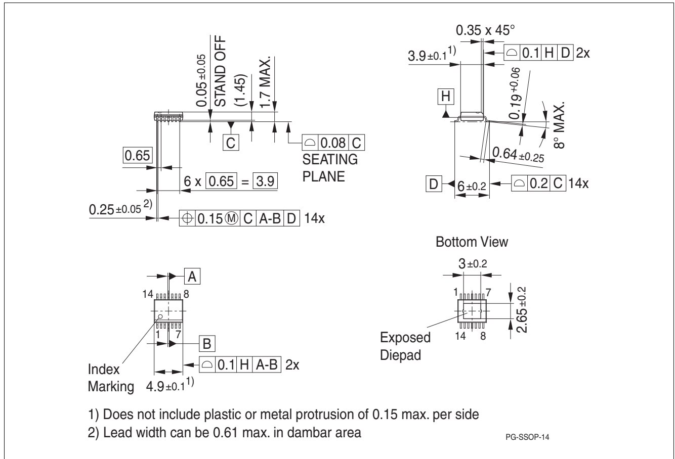
Figure 14 PG-SSOP-14
