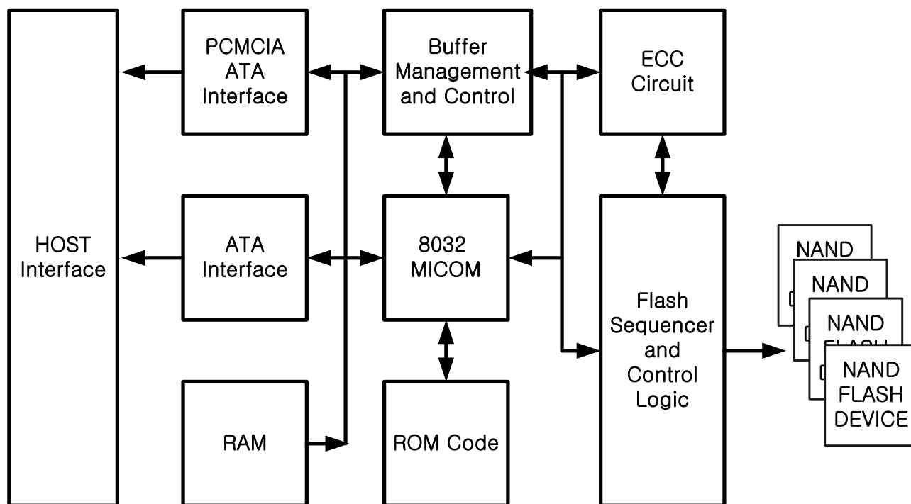
Figure 2.1 Block Diagram
