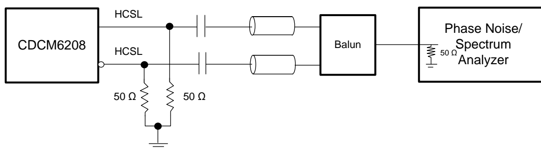
Figure 14. HCSL Output AC Configuration During Device Test
