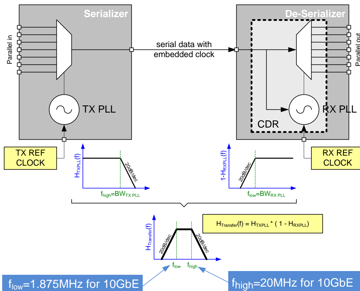
Figure 38. Serial Link Jitter Budget Explanation
