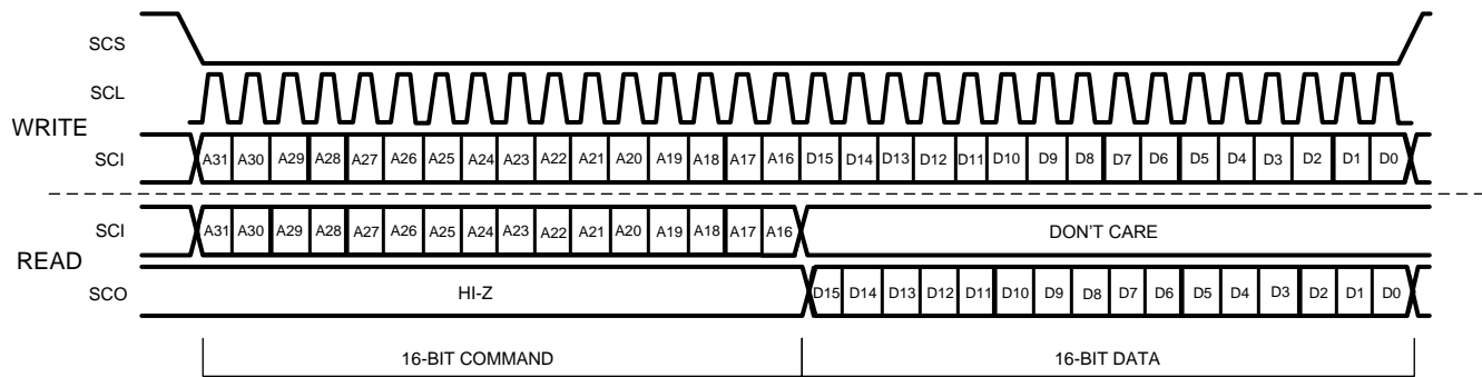
Figure 46. CDCM6208 SPI Port Message Sequencing
