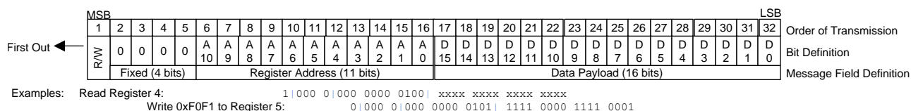
Figure 44. CDCM6208 SPI Message Format
