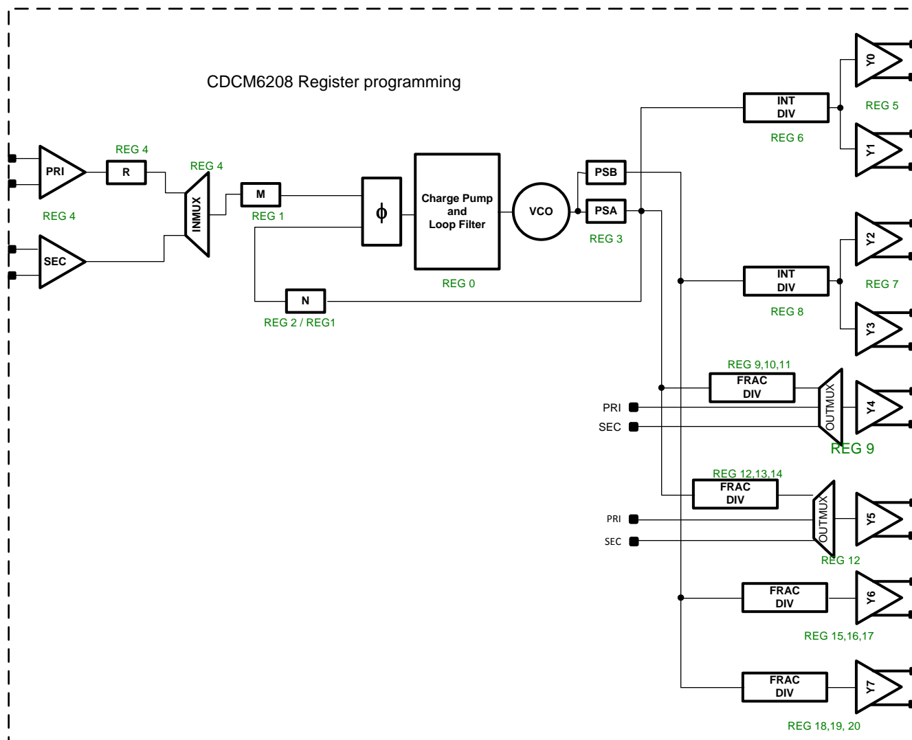
Figure 52. Device Register Map
