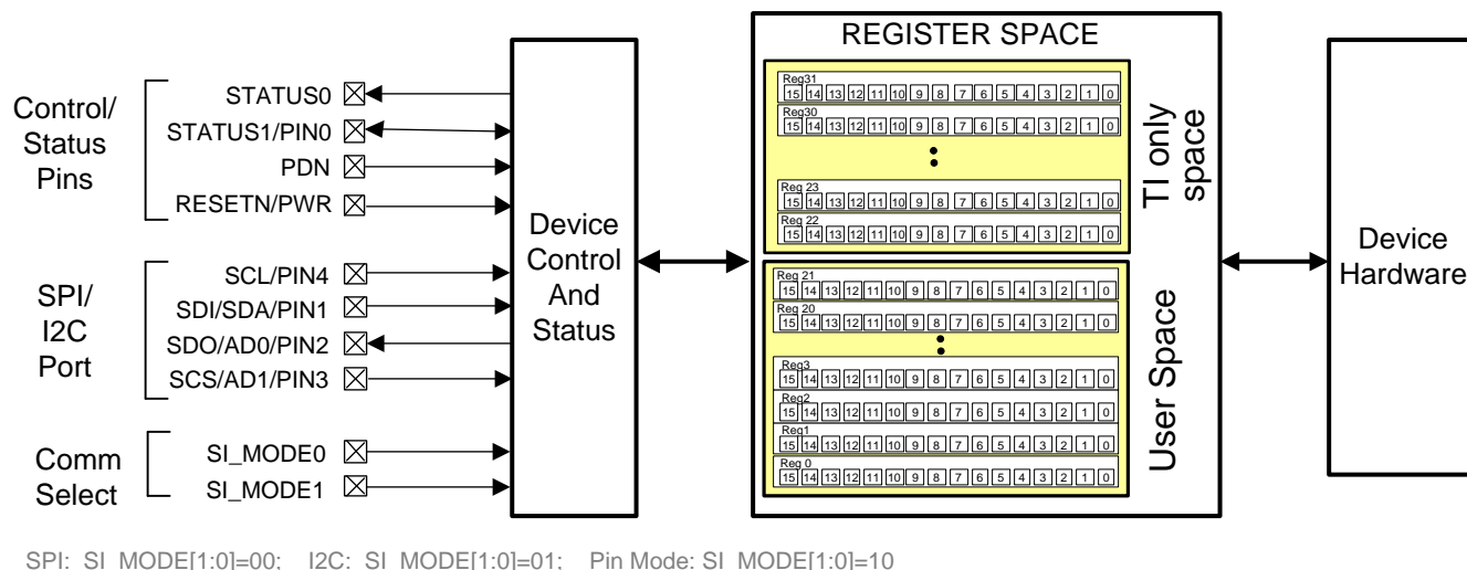
Figure 42. CDCM6208 Interface and Control Block
