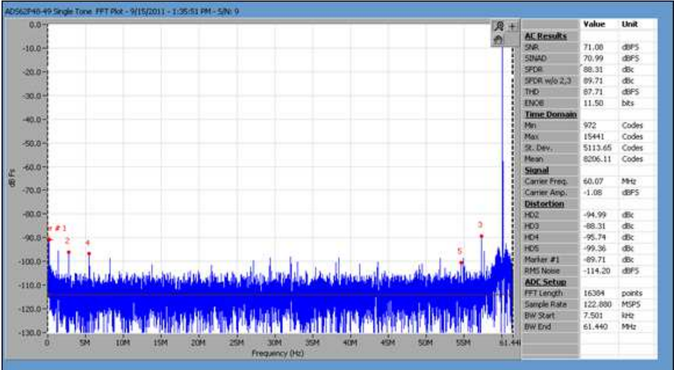
Figure 40. IF = 60 MHz Fclk = 122.88 MHz CDCM6208 driving ADC
