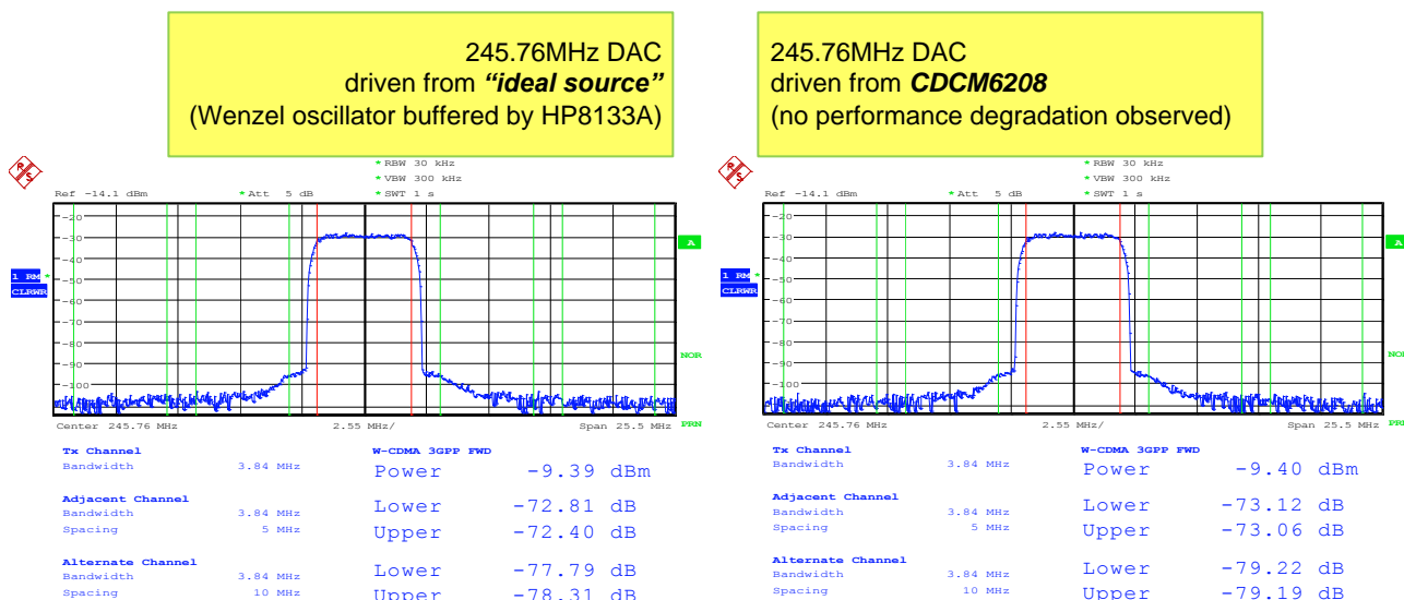
Figure 41. DAC Driven by Lab Source and CDCM6208 in Comparison (Performance Identical)
