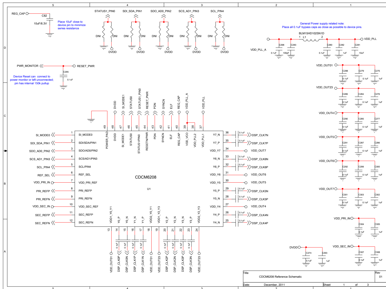
Figure 53. Schematic page 1
