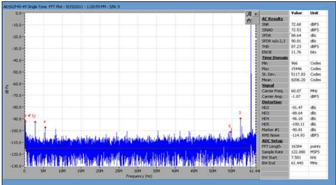
Figure 39. IF = 60 MHz Fclk = 122.88 MHz Baseline (Lab Clk Generator) ADC: ADS62P48-49
