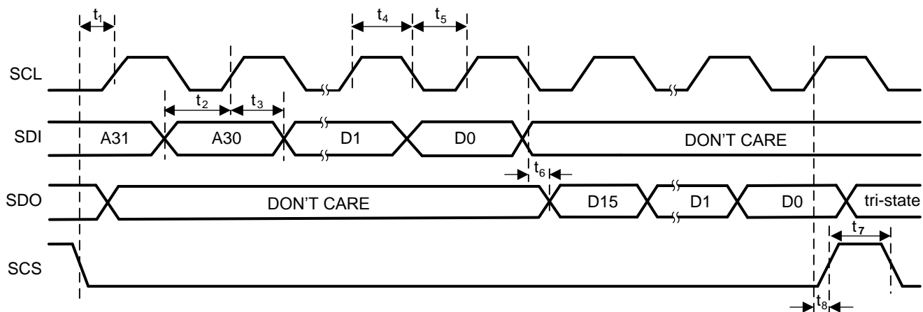
Figure 47. CDCM6208 SPI Port Timing
