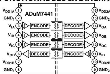
Figure 2. ADuM7441
