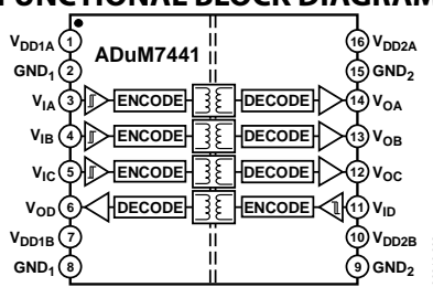
Figure 2. ADuM7441
