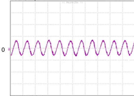
Figure 10: Input reflected ripple current, i_s , through a 12\ \mu\text{H} source inductor at nominal input voltage ( V_{in}=48\text{V} ) and rated load current (20 mA/div, 5us/div)
