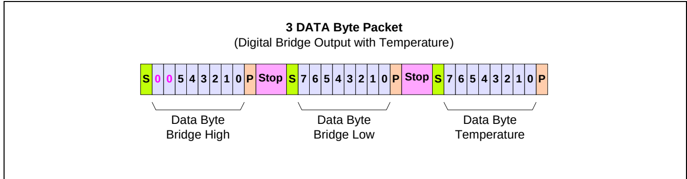
Figure 3.6 Digital Output (NOM) Bridge Readings with Temperature
