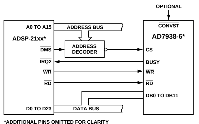
Figure 42. Interfacing to the ADSP-21xx
