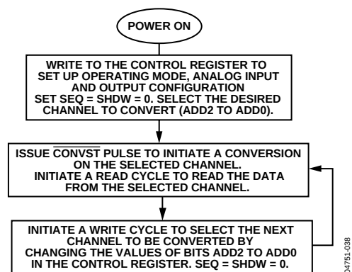
Figure 30. Traditional Multichannel Operation Flow Chart
