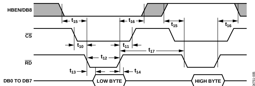
Figure 36. AD7938-6 Parallel Interface—Read Cycle Timing for Byte Mode Operation ( \overline{W/B} = 0 )
