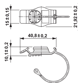
Protective cover, IP67
