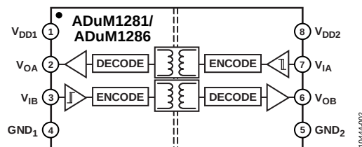
Figure 2. ADuM1281/ADuM1286
