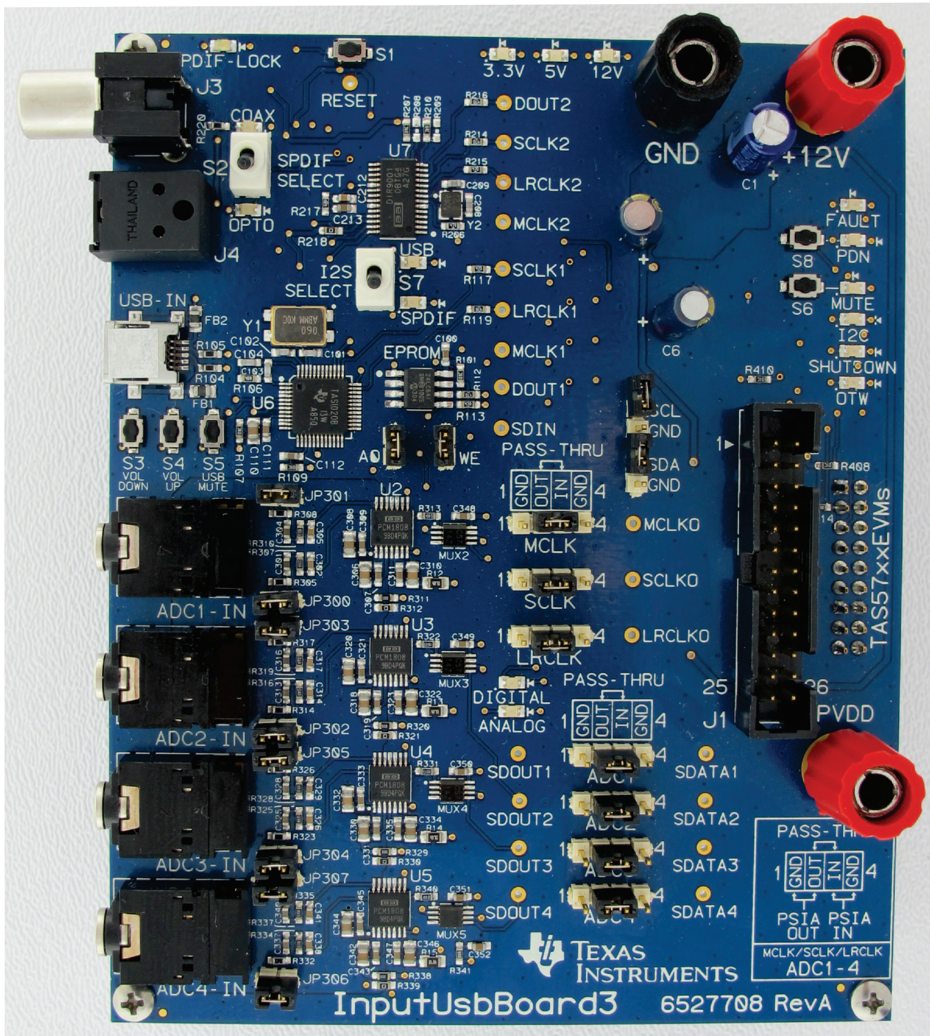
Figure 2. Input-USB Board3
