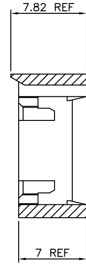
SECTION B-B
